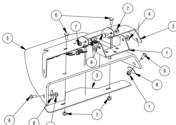
210-6015-98 Discharge Assembly
