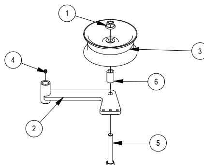
039-6952-23 SD DECK IDLER ASSEMBLY
